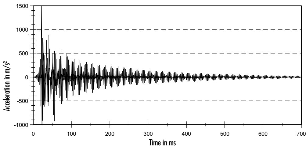
Standard toolholder
